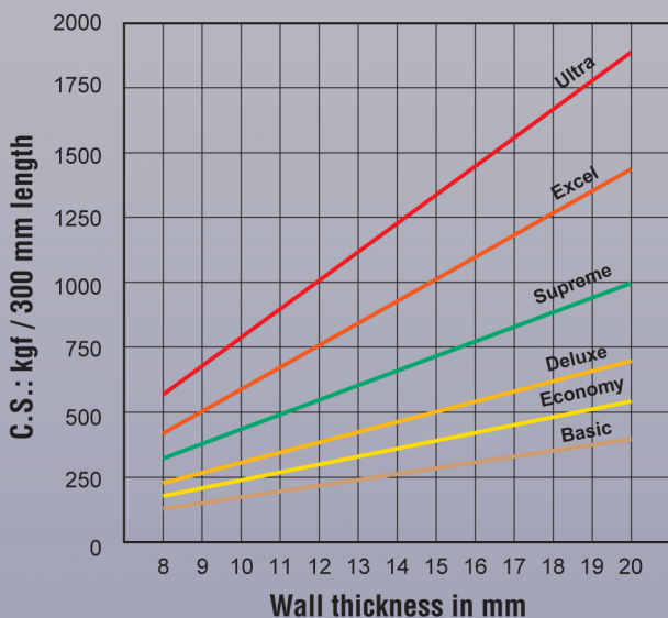
Flat Compression Strength of Paper Cores for dia. 152.40 mm
