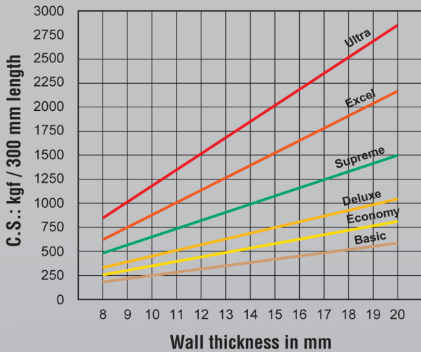
Flat Compression Strength of Paper Cores for dia. 76.20 mm
